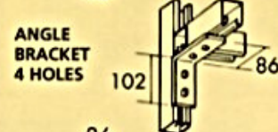
ANGLE BRACKET 4 HOLES
