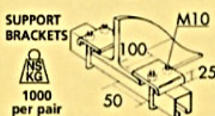
INTERNAL SUPPORT BRACKET
