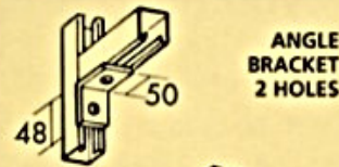
ANGLE BRACKET 2 HOLES
