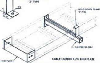
HOLD DOWN CLAMP 'Z' TYPE
